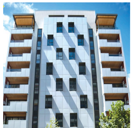
Forte, Melbourne - 10 storeys of cross laminated timber, built in 3 months with just 4 workers and a crane driver.
